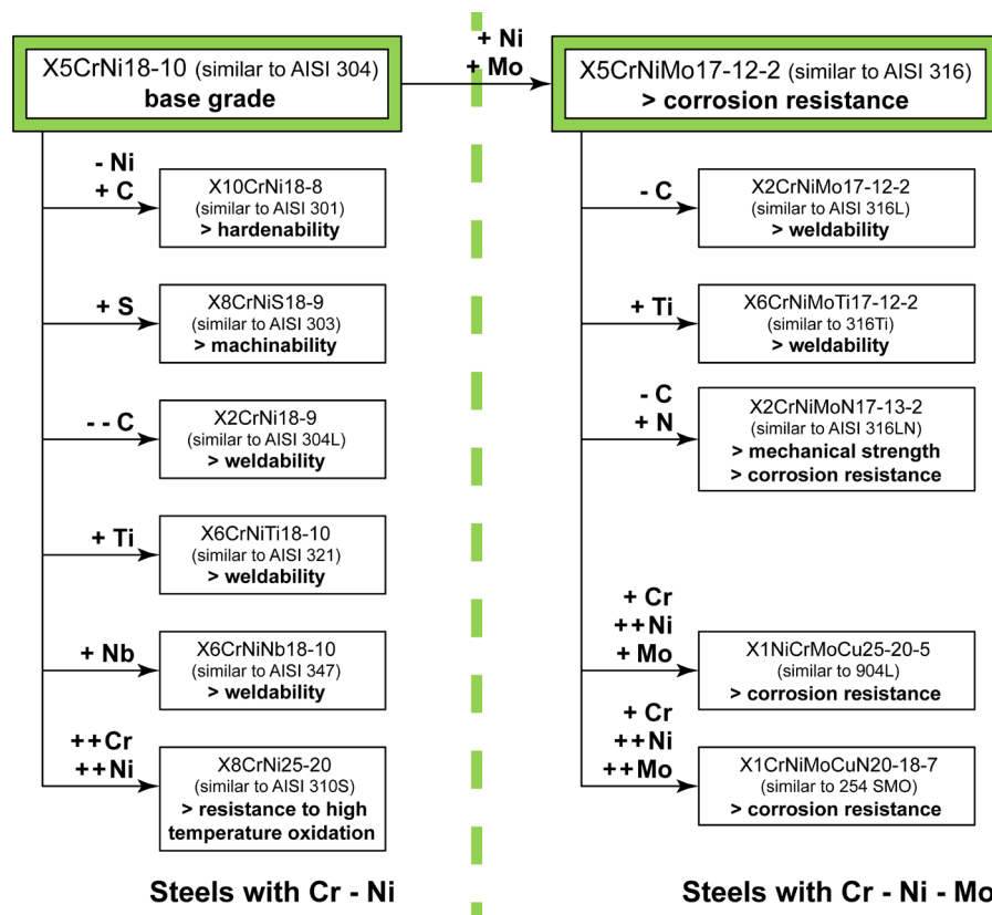
Figure 34 – Main types of chromium-nickel and chromium-nickel-molybdenum austenitic stainless steels starting from EN X5CrNi18-10 (similar to AISI 304) and EN X5CrNiMo17-12-2 (similar to AISI 316).
