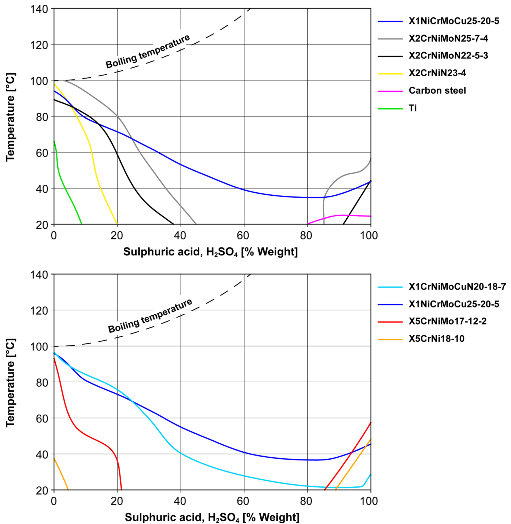
Figure 58 – Iso-corrosion diagrams (0.1mm/year) for some stainless steels in sulphuric acid; the dashed curve indicates the boiling temperature [from Outokumpu 2009].
