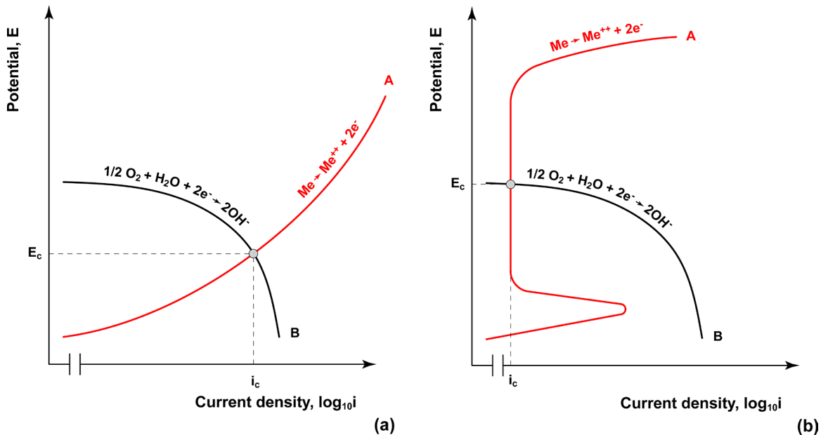
Figure 48 – Schematic representation of potentiodynamic polarisation curves (anodic characteristic A: material - cathodic characteristic B: environment) in aqueous solution 0.05M of H_2SO_4 : (a) material with active behavior, (b) material with active-passive behavior.
