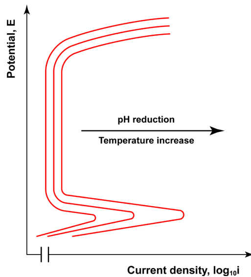
Figure 56 – Effect of temperature and \text{pH} on the anodic polarisation curve of a generic stainless steel.
