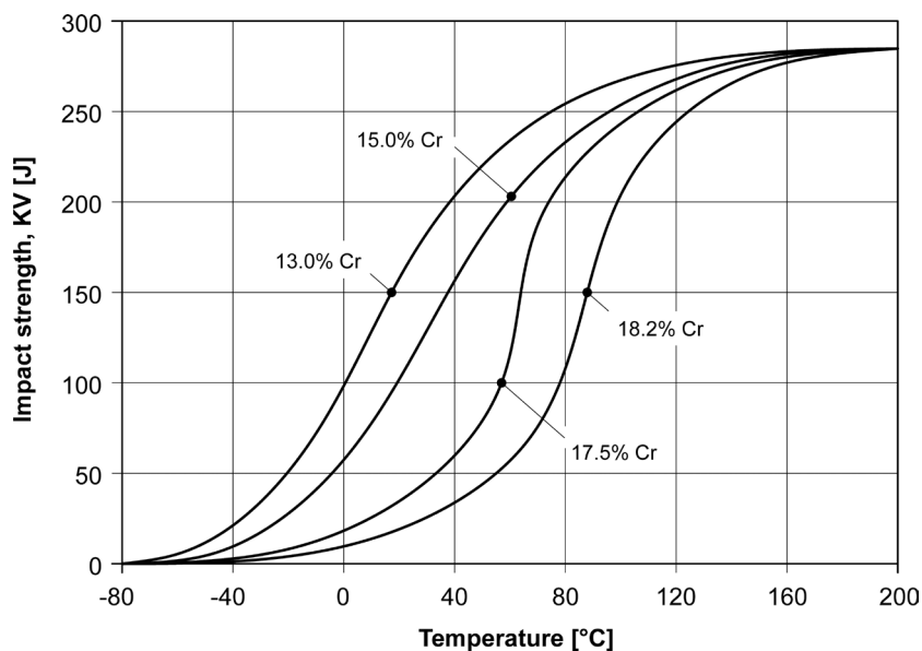
Figure 32 – The effect of chromium on ductile to brittle transition of iron-chromium alloys (carbon is ~0.01%) [from Sedriks 1996].
