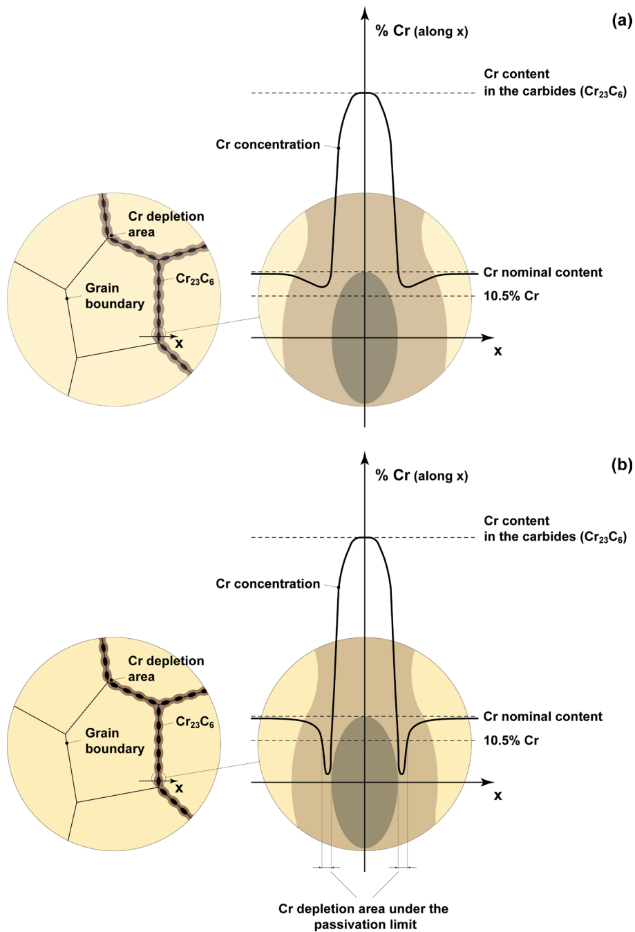
Figure 10 – Chromium concentrations at grain boundary after chromium carbide precipitation: (a) ferritic stainless steel (high diffusivity of chromium), (b) austenitic stainless steel (low diffusivity of chromium).
