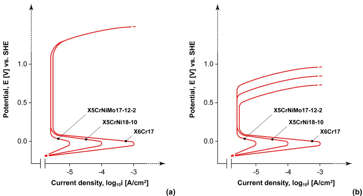
Figure 54 – Schematic representation of potentiodynamic polarisation curves for three stainless steels in acid solutions contaminated with chlorides: (a) 0.05 M solution of sulphuric acid, (b) 0.05 M solution of sulphuric acid and 0.1 M solution of sodium chloride [from Talbot and Talbot 1998].
