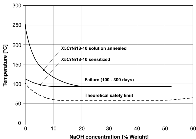
Figure 80 – Effect of temperature and sodium hydroxide concentration ( \text{NaOH} ) on caustic SCC resistance of austenitic stainless steel grade EN X5CrNi18-10 [from Lacombe 1993].
