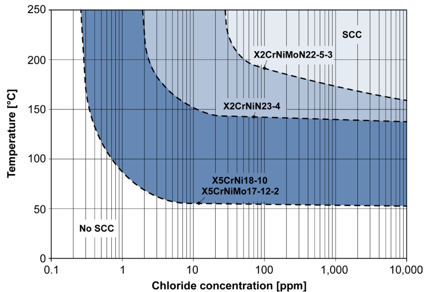
Figure 79 – Effect of temperature and chloride concentration on SCC resistance of some austenitic and austenitic-ferritic stainless steels [from Sedriks 1996].
