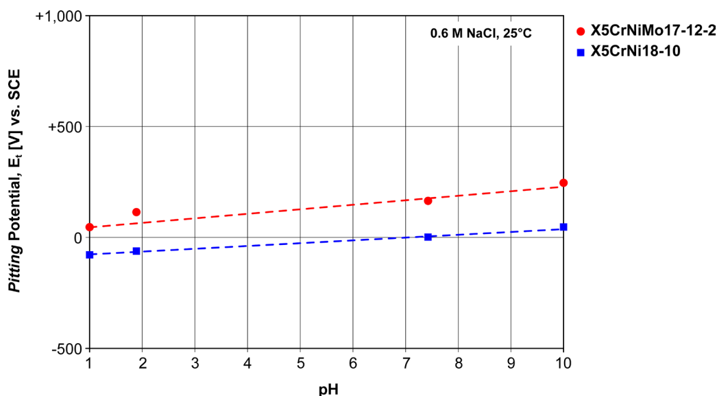
Figure 66 – Pitting potential according to pH for austenitic stainless steel grades EN X5CrNi18-10 and EN X5CrNiMo17-12-2 in aqueous solution 0.6 M of NaCl at 25°C [from Shirer 1994].
