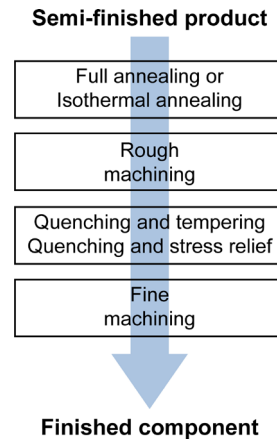
Figure 18 – Technological process required to produce a component in martensitic stainless steel.
