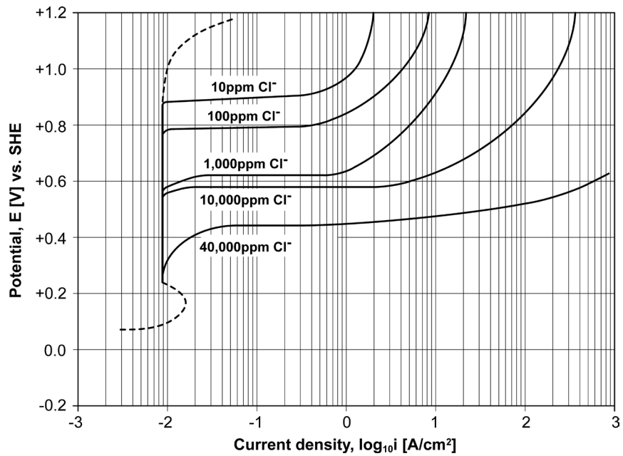
Figure 55 – Potentiodynamic polarisation curves for stainless steel grade EN X5CrNi18-10 in water at 25°C contaminated with different levels of chlorides, \text{Cl}^- [from Stansbury and Buchanan 2000].
