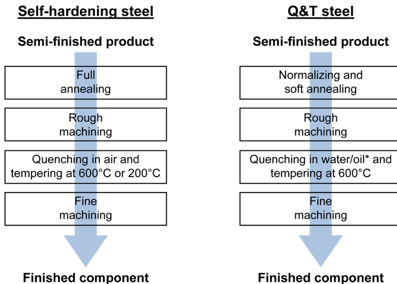
Figure 15.4 – Comparison of the manufacturing cycles to obtain a component from a self-hardening steel (on the left) or from a Q&T steel (on the right).
