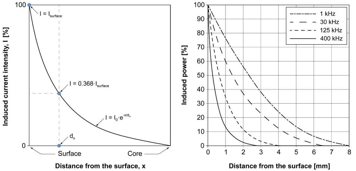
Figure 14.13 – (on the left) Induced current distribution on the part surface due to the skin effect [from Davies and Simpson 1979] - (on the right) Induced power distribution in the part as a function of the current frequency [from ASM-H.4 1991].
