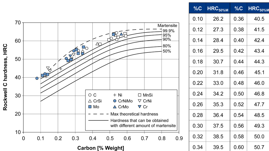
Figure 13.1 – HRC hardness trend as a function of carbon content and martensite percentage for quenched and tempered steels with different chemical compositions [from Liščič et al. 1992].
