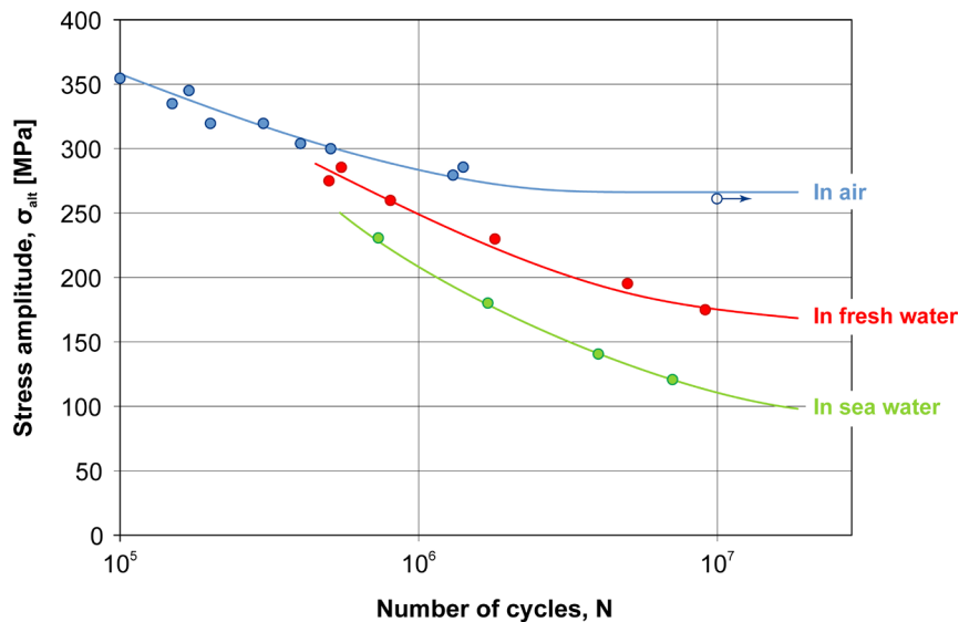
Figure 6.18 – Trend of Wöhler curves in rotating bending fatigue conditions ( R = -1 ) for an EN C45 steel grade ( Y_S = 410 MPa; UTS = 630 MPa) in air, in freshwater and in seawater [from Endo and Miyao 1958].
