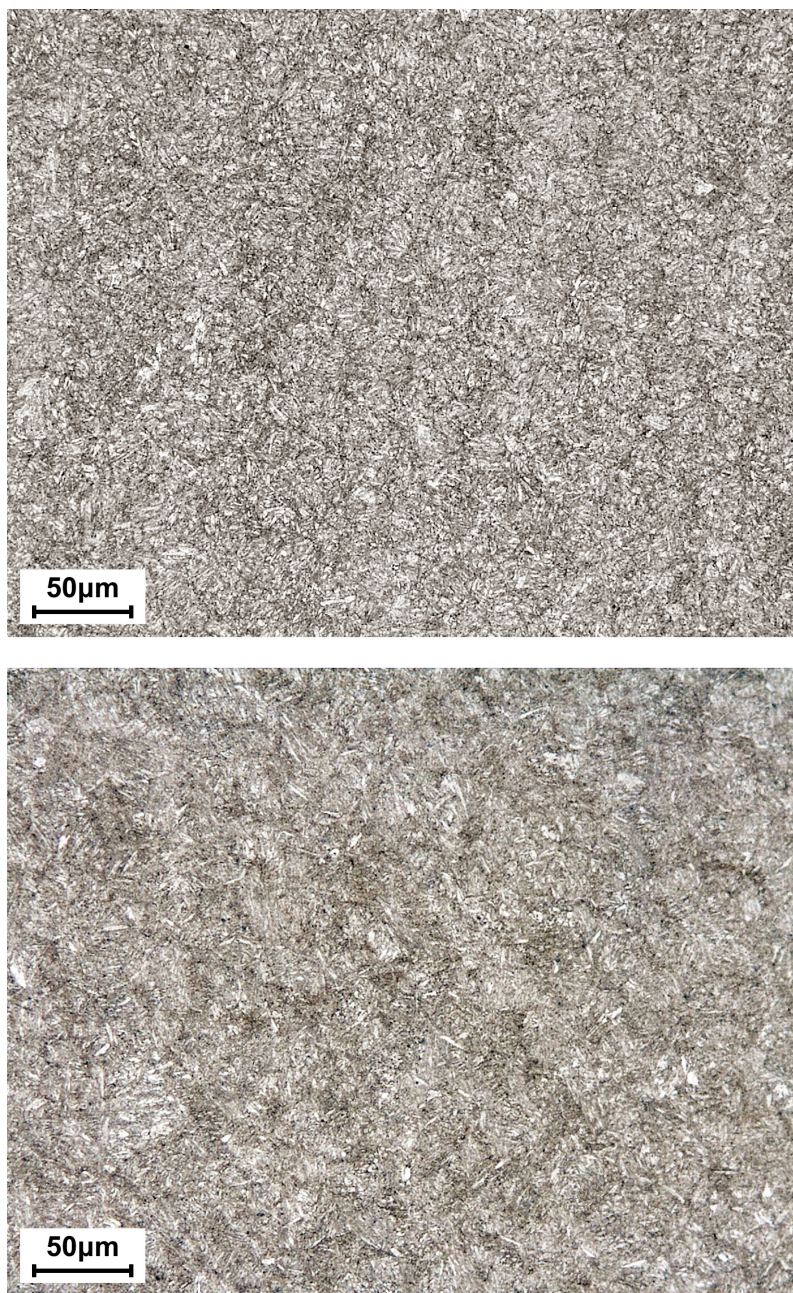
Figure 13.2 – Metallographic appearance of the tempered martensitic structure of steel grades EN 42CrMo4 (top) and EN 36CrNiMo4 (bottom) [Exova S.r.l. Laboratories - Crema, Italy].
