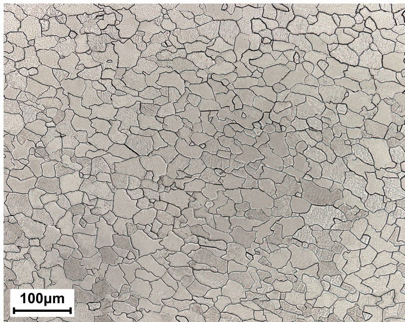
Figure 9.11 – Metallographic appearance of cold forming steel grade EN DD14. Notice the fully recrystallized ferritic structure; etching agent: Nital 2%. [Laboratories of the Department of Mechanical Engineering of Politecnico di Milano – Milan, Italy].
