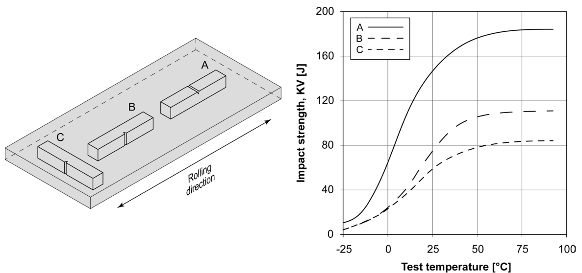
Figure 4.16 – Impact energy transition curves for steel with C = 0.012%. Effect of the fibre pattern in a plate after hot deformation depending on specimen sectioning direction [from Puzak et al. 1952].
