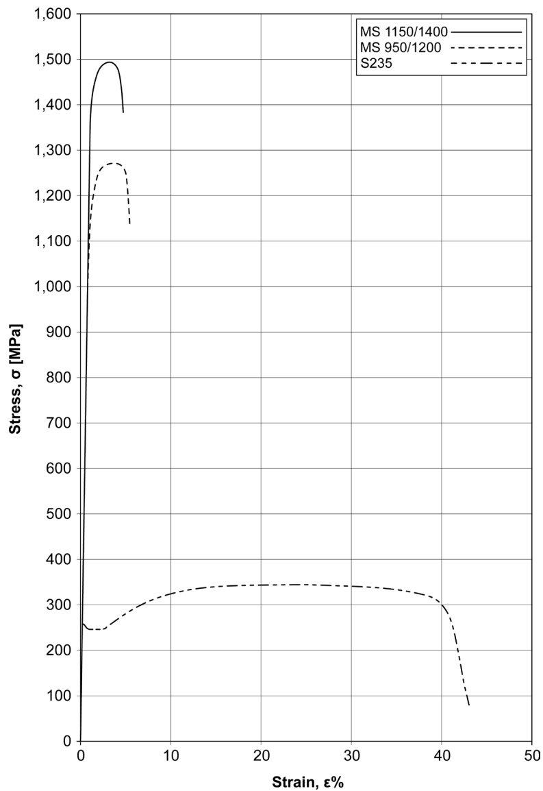
Figure 11.7 – Stress/strain curves for some martensitic steels (identified by the letters MS followed by their minimum YS and UTS values) compared to a generic EN S235 steel [from Keeler et al. 2017]
