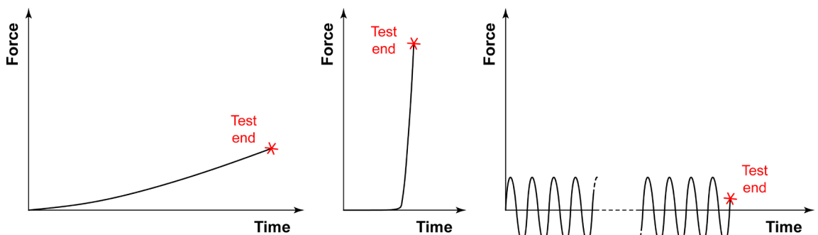
Figure 1.1 – Schematic of force trends as applied over time until specimen breakage for all test types.
