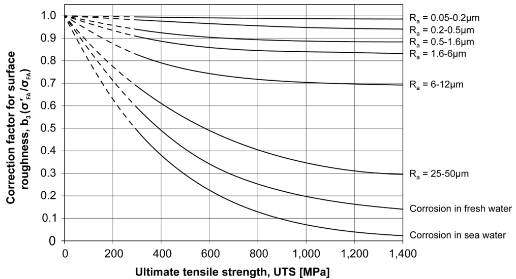
Figure 6.24 – Trend of the surface finish coefficient b_s that enables defining the component fatigue limit ( \sigma'_{FA} ) starting from the material fatigue limit ( \sigma_{FA} ) as a function of component roughness. The entry value plotted in the abscissa axis is steel Ultimate Tensile Strength [from Brand et al. 1991].
