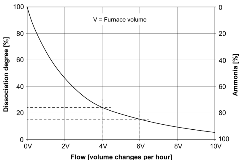
Figure 18.12 – Correlation of ammonia dissociation degree and flow rate in the process furnace in a 100% \text{NH}_3 atmosphere [from Herring 2011].
