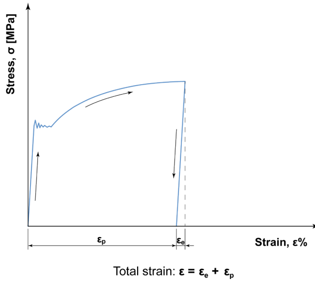
Figure 2.8 – Schematic of the stress-strain curve ( \sigma - \varepsilon ) for a general-purpose structural steel type EN S275. The tensile test was discontinued and the stress level brought back to zero at the plastic strain region.
