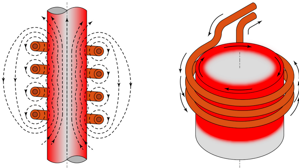
Figure 14.7 – (on the left) Trend of the magnetic field induced in a steel round bar placed into a solenoid inductor through which alternate current is flowing; (on the right) Electric current trend in the inductor and in the round bar [from Thelning 1975].
