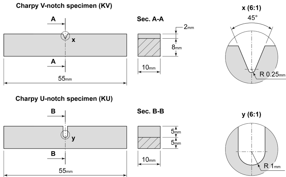
Figure 4.1 – Geometrical characteristics of V-notch and U-notch impact test specimens
