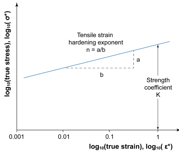
Figure 2.13 – Representation of Hollomon's equation in a bilogarithmic graph \log_{10}(\sigma^*) - \log_{10}(\varepsilon^*) .
