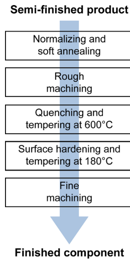
Figure 14.6 – Schematic of the manufacturing cycle for a component obtained from surface hardened Q&T steel.
