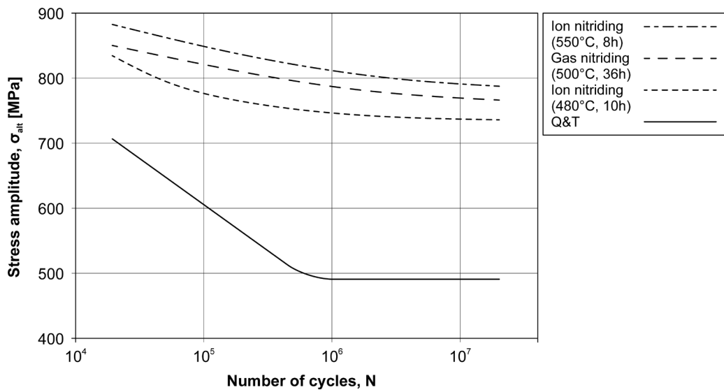
Figure 6.19 – Wöhler curves in rotating bending conditions ( R = -1 ) for an EN 42CrMo4 steel grade ( Y_S = 780 MPa; UTS = 980 MPa), after quenching and tempering and after quenching and tempering followed by nitriding in different modes [from ASM-H.1 1991].
