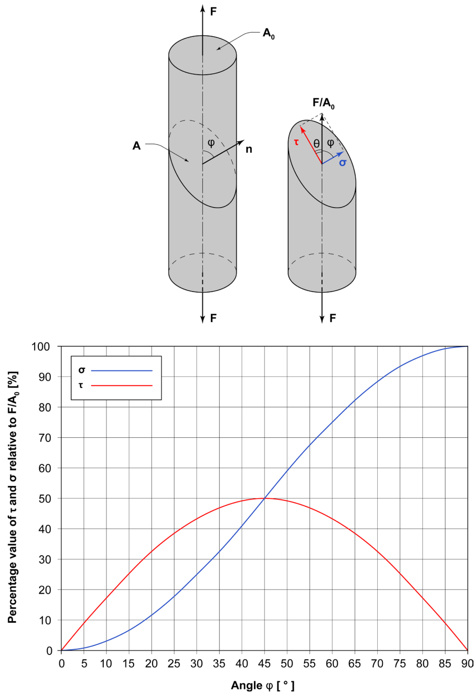
Figure 5.1 – Trend of average stresses that are tangential ( \tau ) and normal ( \sigma ) to plane A inclined relative to the axis in accordance with angles \theta and \phi . The values of \tau and \sigma are expressed as percentages of the average stress generated by the force F on the surface A_0 , this being normal to the grain axis [from Brooks et al. 1993]
